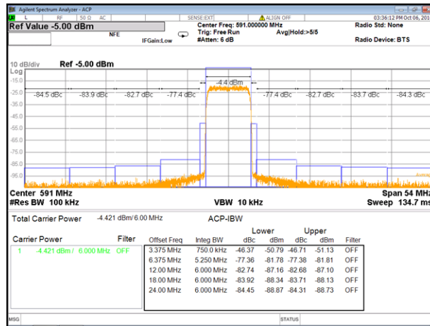
Figure 144. ACPR Performance of 6 MHz Single Carrier at 591 MHz
