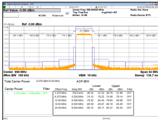
Figure 145. ACPR performance of 6 MHz Single Carrier at 998 MHz
