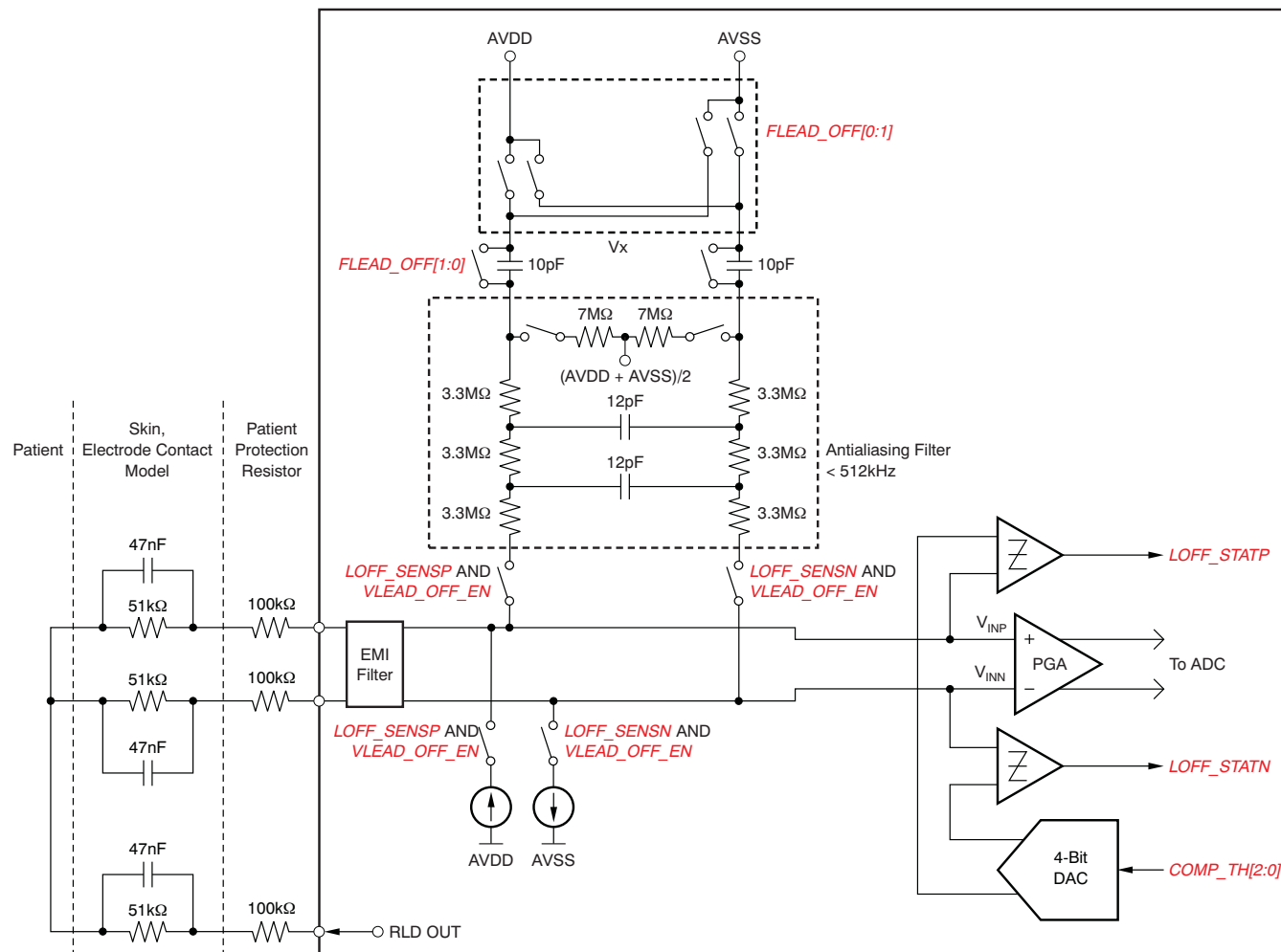
Figure 46. Lead-Off Detection
