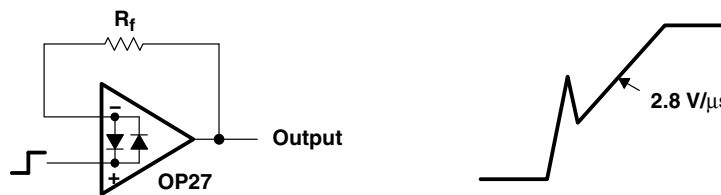
Figure 31. Pulsed Operation
