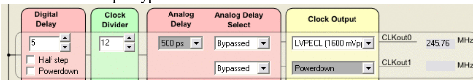
Figure 6: Setting Digital Delay, Clock Divider, Analog Delay, and Output Format for CLKout0
