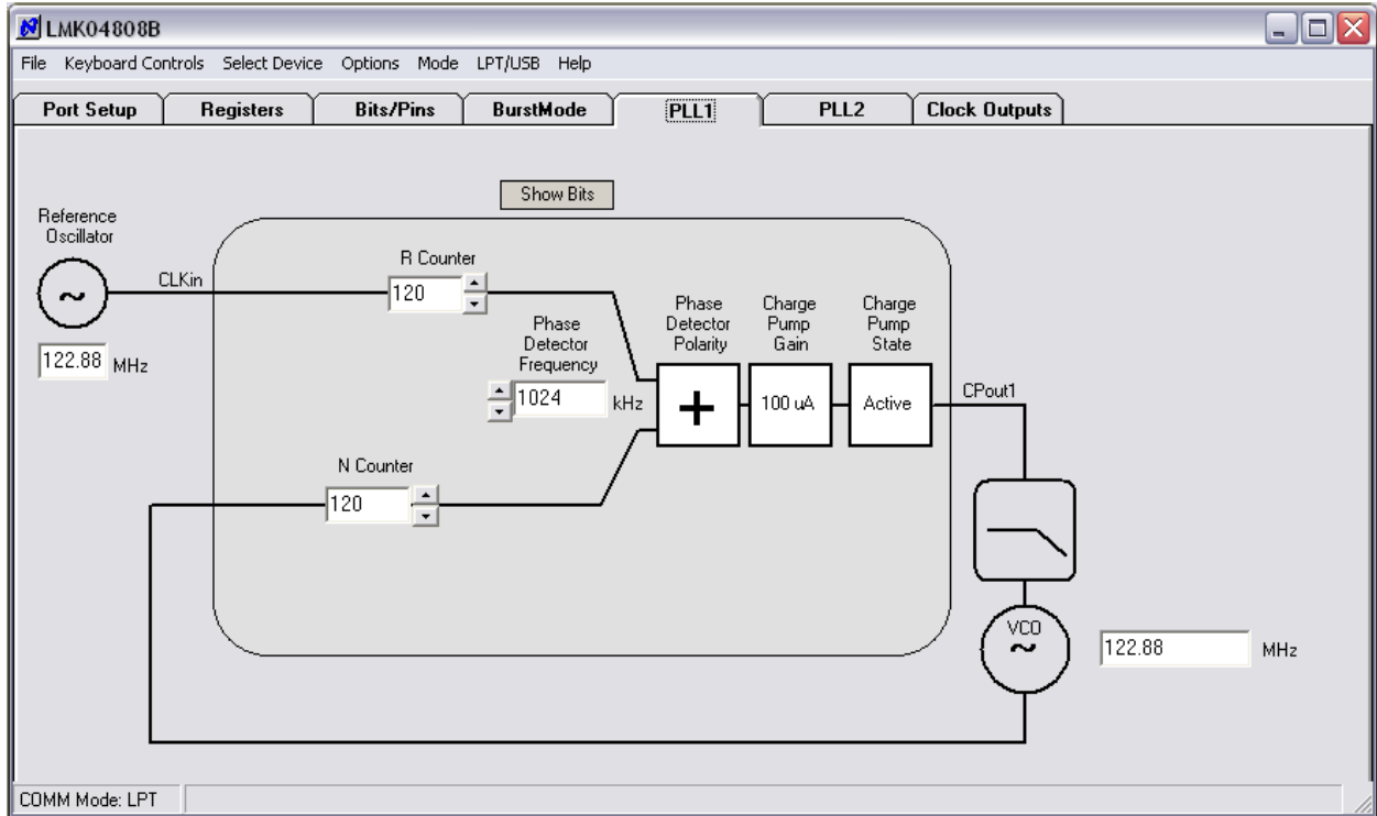
Figure 11: PLL1 tab
