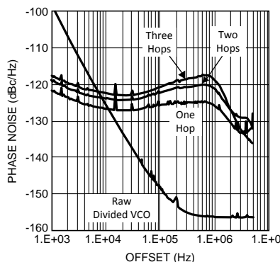
Figure 6. Determining Which Loop Bandwidth to Use
