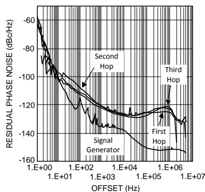
Figure 3. Calculated Residual Phase Noise
