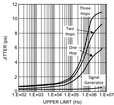
Figure 4. Jitter as a Function of UpperLimit
