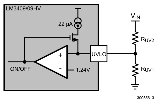
FIGURE 8. UVLO Circuit
