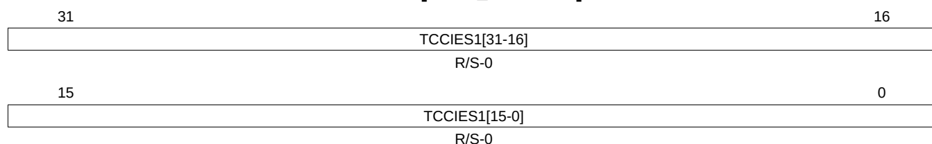
Figure 26-95. Transfer to Communication Controller Interrupt Enable Set 1 (TCCIES1) [offset_TU = 120h]
