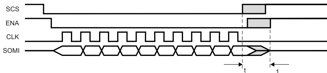
Figure 28-47. Transmit-Data-Finished-to-ENA-Inactive-Timeout
