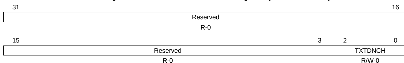
Figure 32-41. Transmit Teardown Register (TXTEARDOWN)
