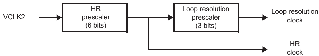
Figure 23-7. Prescaler Configuration
