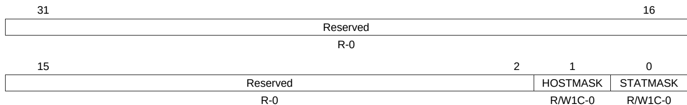
Figure 32-58. MAC Interrupt Mask Clear Register (MACINTMASKCLEAR)
