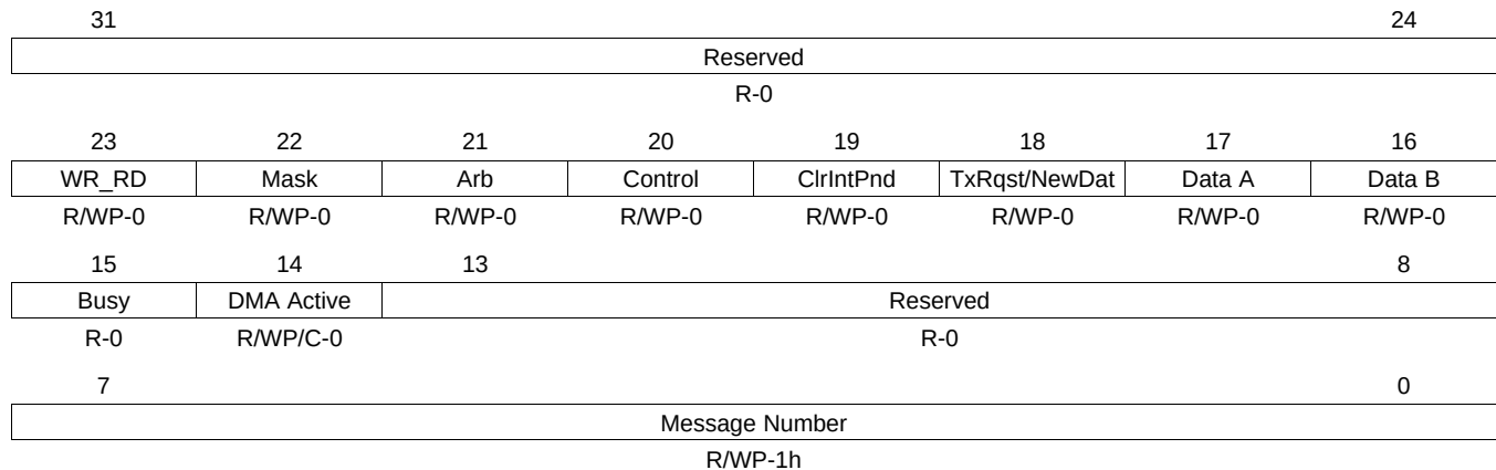
Figure 27-51. IF1 Command Registers (DCAN IF1CMD) [offset = 100h]
