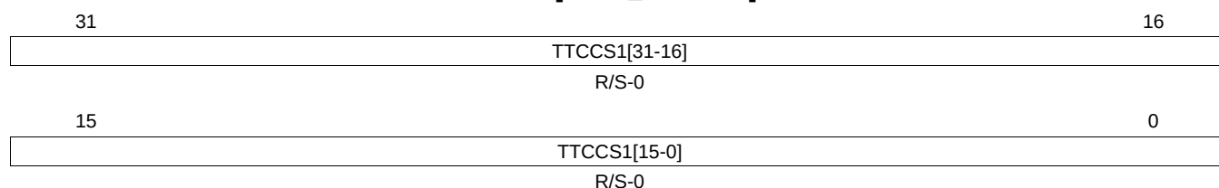
Figure 26-63. Trigger Transfer to Communication Controller Set 1 (TTCCS1) [offset_TU = A0h]
