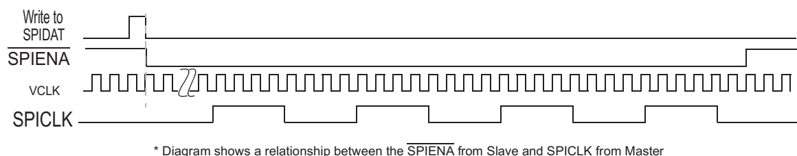
Figure 28-86. SPI/MibSPI Pins During Slave Mode 4-pin with \overline{\text{SPIENA}} Configuration
