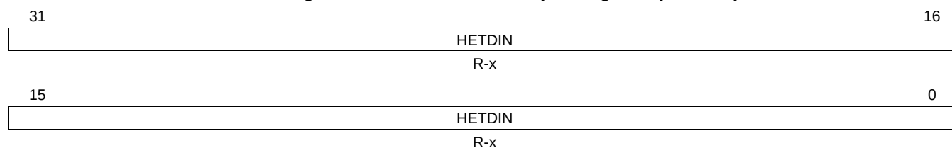
Figure 23-53. N2HET Data Input Register (HETDIN)
