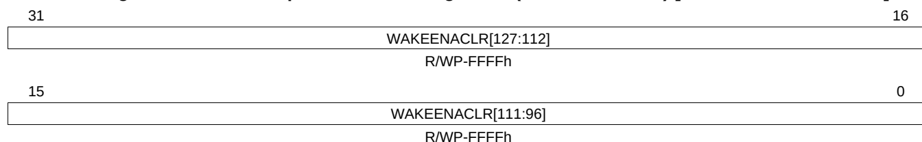
Figure 15-40. Wake-Up Enable Clear Register 3 (WAKEENACLR3) [Address = FFFF FE6Ch]
