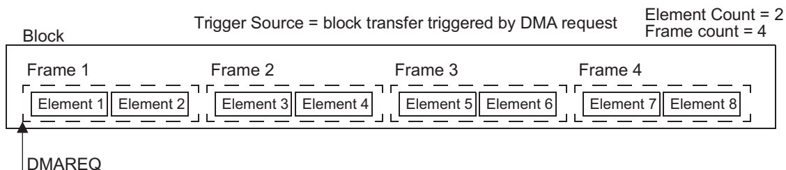
Figure 16-3. Example of a DMA Transfer Using Block Trigger Source
