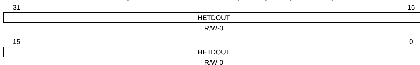
Figure 23-54. N2HET Data Output Register (HETDOUT)
