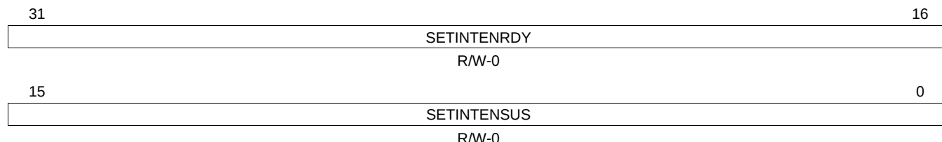
Figure 28-56. TG Interrupt Enable Set Register (TGITENST) [offset = 74h]
