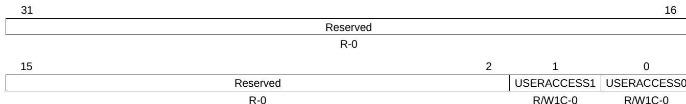
Figure 32-31. MDIO User Command Complete Interrupt (Unmasked) Register (USERINTRAW)
