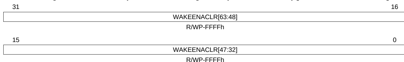
Figure 15-38. Wake-Up Enable Clear Register 1 (WAKEENACLR1) [Address = FFFF FE64h]
