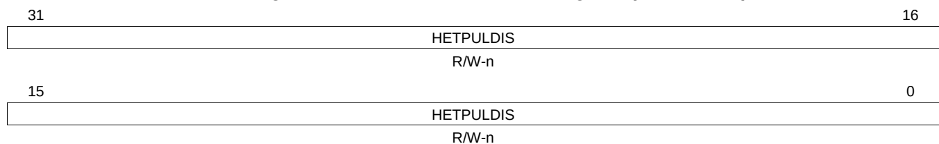
Figure 23-58. N2HET Pull Disable Register (HETPULDIS)
