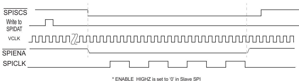
Figure 28-87. SPI/MibSPI Pins During Slave Mode in 5-pin Configuration - (Single Slave)
