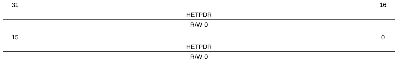
Figure 23-57. N2HET Open Drain Register (HETPDR)
