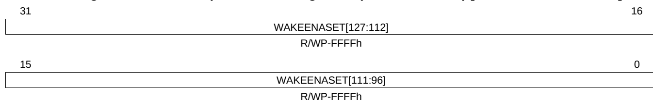
Figure 15-36. Wake-Up Enable Set Register 3 (WAKEENASET3) [Address = FFFF FE5Ch]
