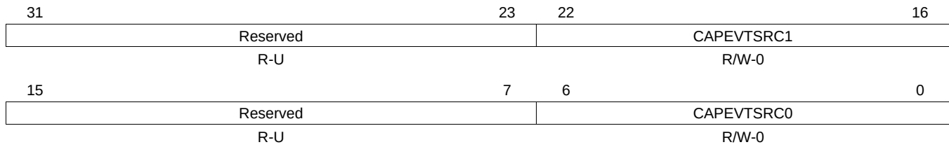
Figure 15-43. Capture Event Register (CAPEVT) [Address = FFFF FE78h]
