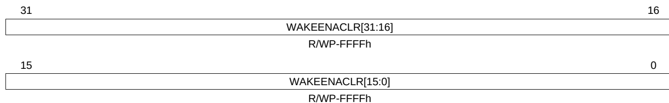
Figure 15-37. Wake-Up Enable Clear Register 0 (WAKEENACLR0) [Address = FFFF FE60h]
