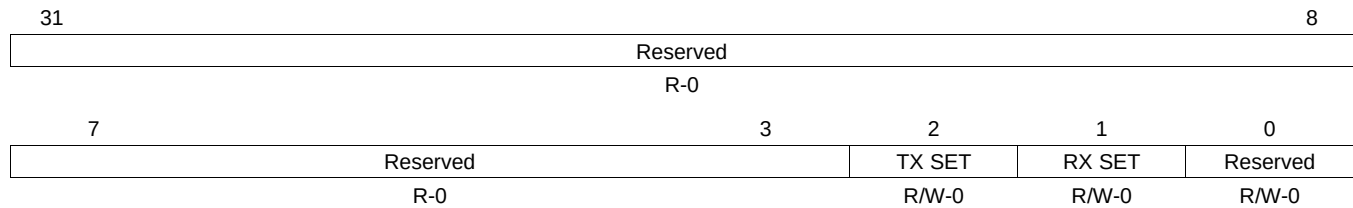
Figure 30-26. SCI Pin I/O Control Register 4 (SCIPIO4) [offset = 4Ch]
