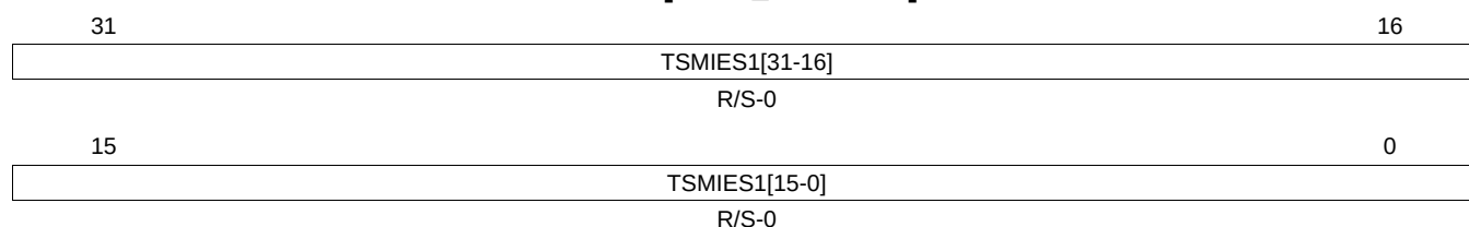
Figure 26-87. Transfer to System Memory Interrupt Enable Set 1 (TSMIES1) [offset_TU = 100h]
