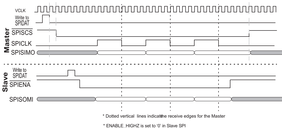
Figure 28-84. SPI/MibSPI Pins During Master/Slave Mode with 5-pin Configuration
