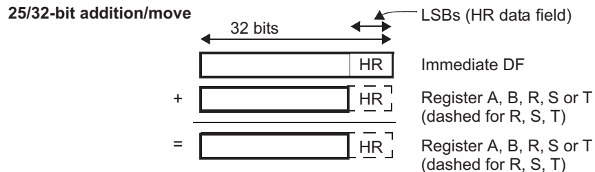
Figure 23-85. ADM32 Add and Move Operation for IM&REGTOREG (Case 00)
