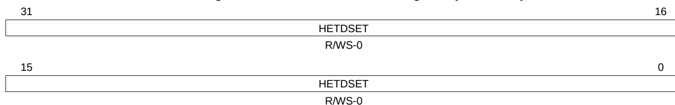
Figure 23-55. N2HET Data Set Register (HETDSET)
