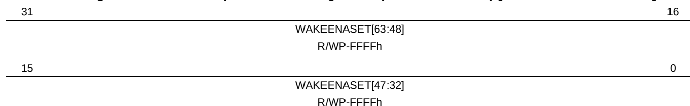
Figure 15-34. Wake-Up Enable Set Register 1 (WAKEENASET1) [Address = FFFF FE54h]
