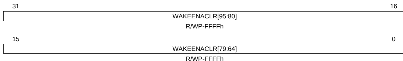
Figure 15-39. Wake-Up Enable Clear Register 2 (WAKEENACLR2) [Address = FFFF FE68h]
