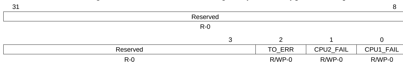
Figure 8-9. Self-Test Fail Status Register (STCFSTAT) [offset = 18h]
