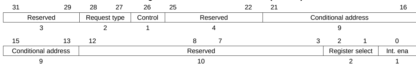
Figure 23-101. DJZ Control Field (C31:C0)
