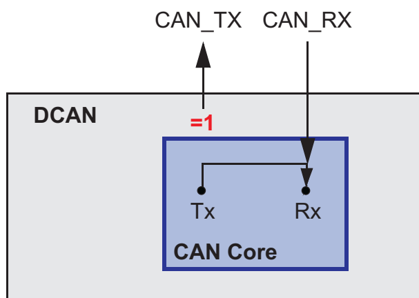
Figure 27-15. CAN Core in Silent Mode
