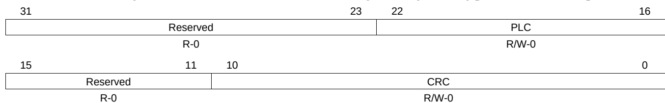
Figure 26-175. Write Header Section Register 2 (WRHS2) [offset_CC = 504h]
