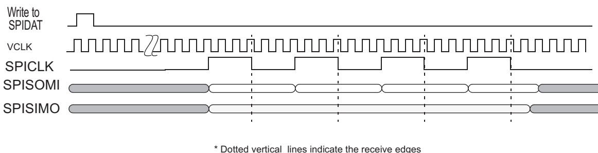
Figure 28-85. SPI/MibSPI Pins During Slave Mode 3-pin Configuration
