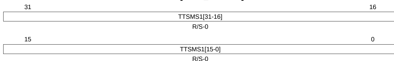
Figure 26-55. Trigger Transfer to System Memory Set 1 (TTSMS1) [offset_TU = 80h]
