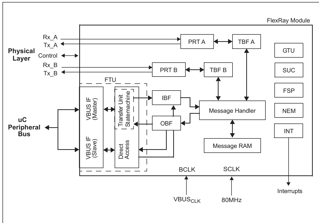
Figure 26-1. Block Diagram
