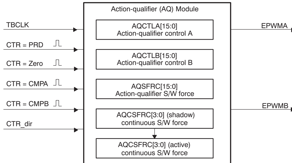
Figure 19-18. Action-Qualifier Submodule Inputs and Outputs
