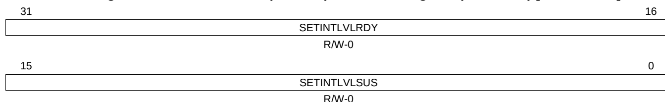
Figure 28-58. Transfer Group Interrupt Level Set Register (TGITLVST) [offset = 7Ch]
