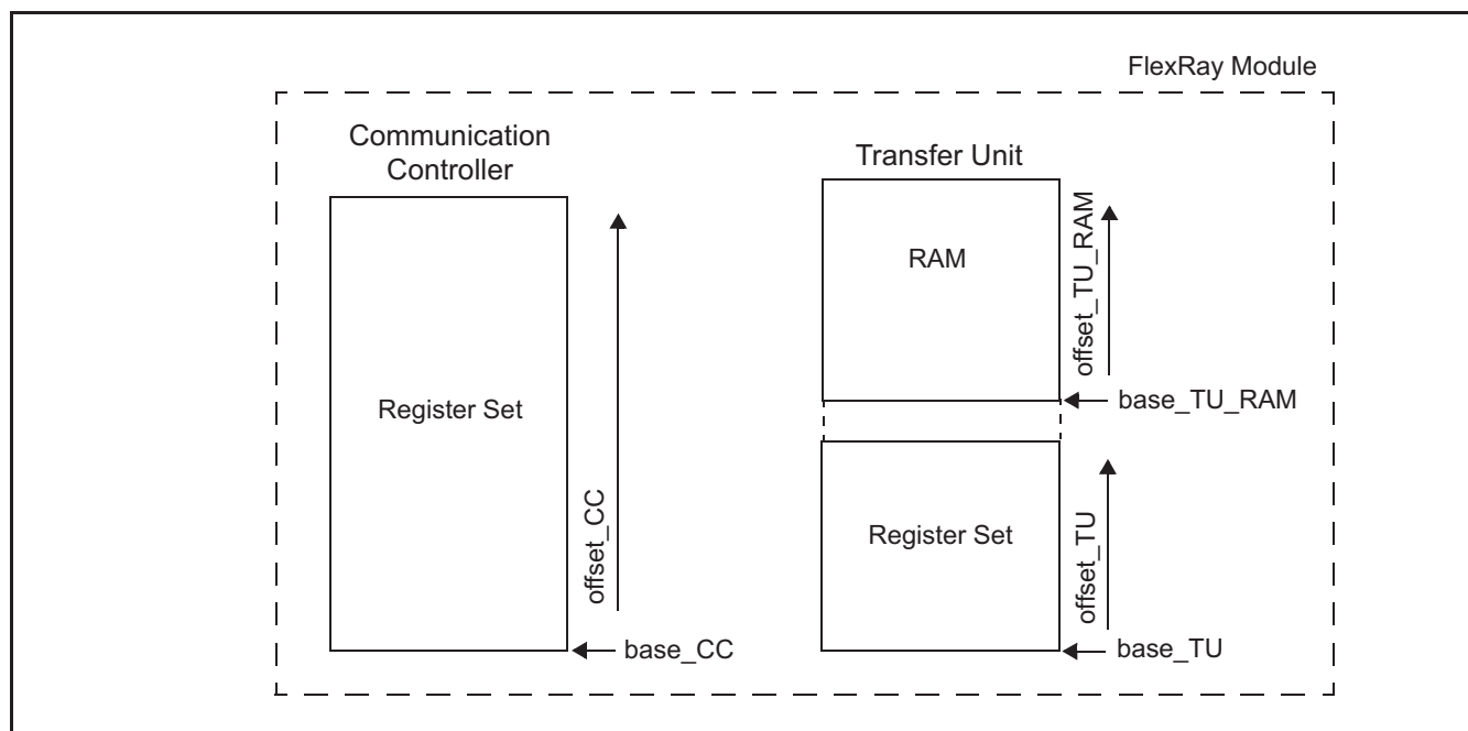
Figure 26-2. FlexRay Module Blocks
