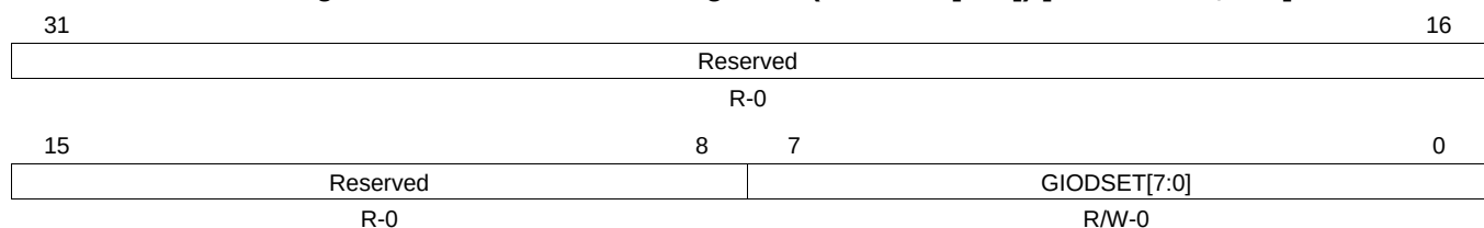
Figure 25-20. GIO Data Set Registers (GIODSET[A-B]) [offset = 40h, 60h]
