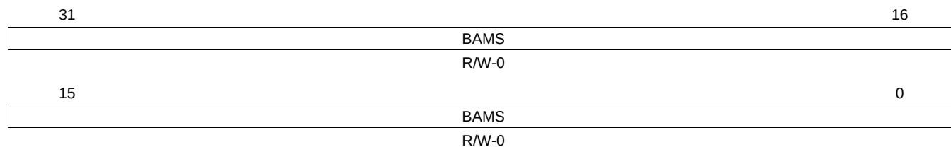
Figure 26-39. Base Address of Mirrored Status (BAMS) [offset_TU = 2Ch]
