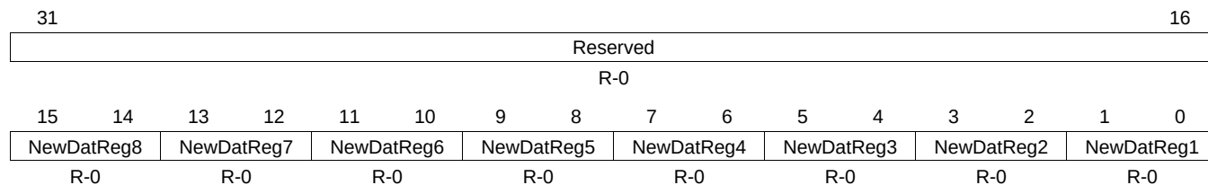
Figure 27-32. New Data X Register (DCAN NWDAT X) [offset = 98h]
