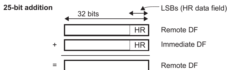
Figure 23-77. ADCNST Operation If Remote Data Field[31:7] Is Not Zero
