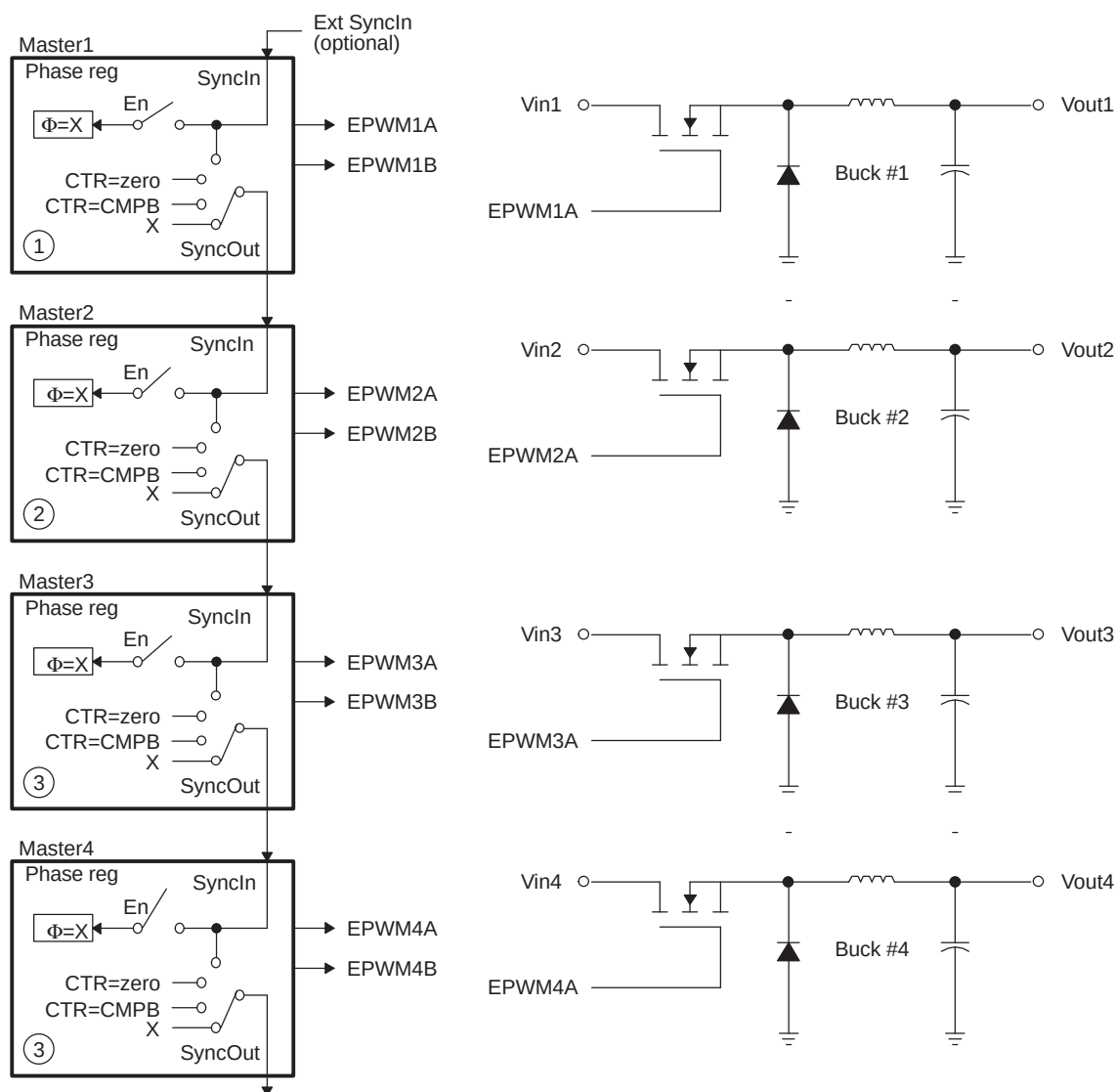
Figure 19-53. Control of Four Buck Stages. Here F_{PWM1} \neq F_{PWM2} \neq F_{PWM3} \neq F_{PWM4}
