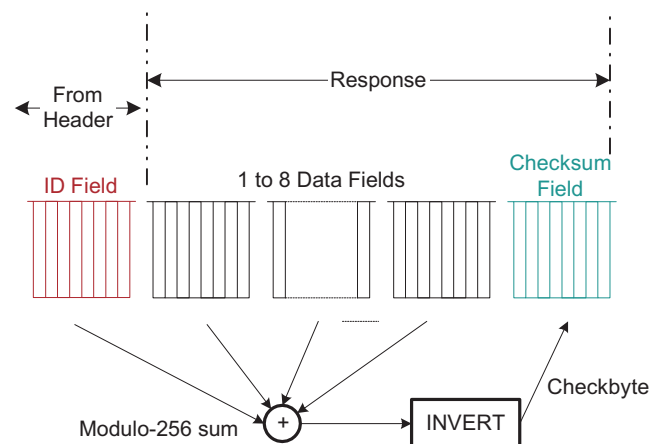
Figure 29-23. LIN 2.0-Compliant Checksum Generation at Transmitting Node
