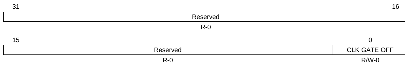
Figure 18-5. POM Clock Gate Control Register [address = FFA0 4008h]
