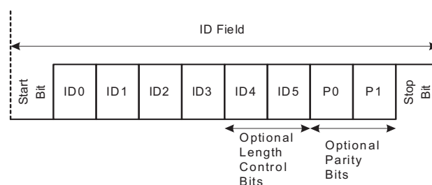
Figure 29-16. ID Field
