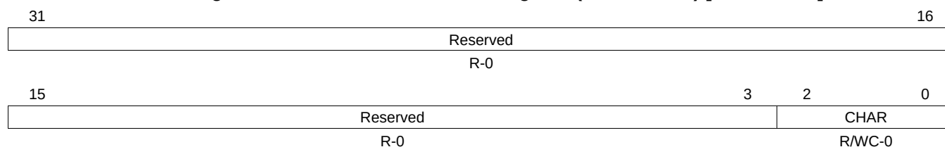
Figure 30-17. SCI Format Control Register (SCIFORMAT) [offset = 28h]
