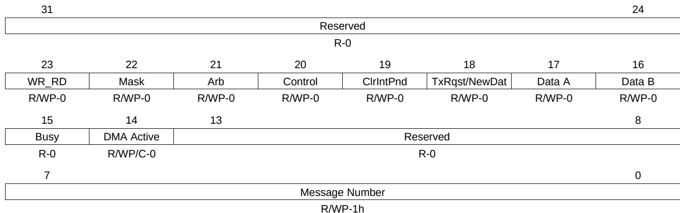
Figure 27-52. IF2 Command Registers (DCAN IF2CMD) [offset = 120h]
