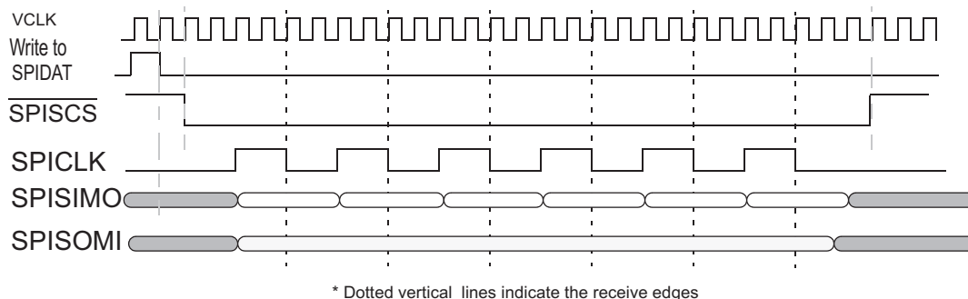
Figure 28-82. SPI/MibSPI Pins During Master Mode 4-pin with \overline{\text{SPISCS}} Configuration
