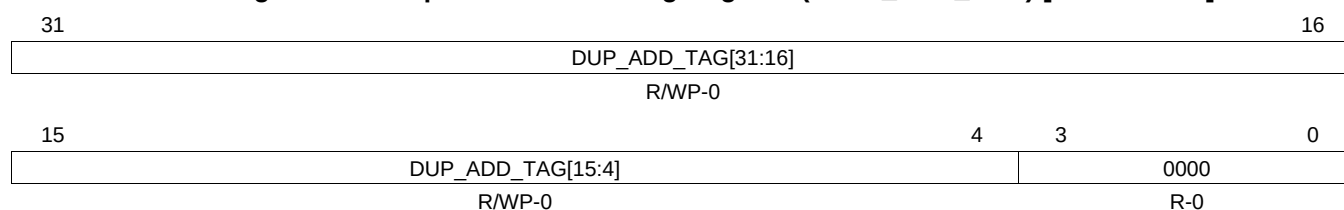
Figure 5-17. Duplicate Address Tag Register (FDUP_ADD_TAG) [offset = 2Ch]
