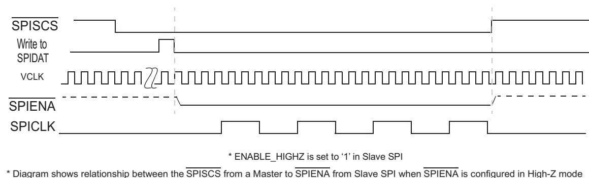
Figure 28-88. SPI/MibSPI Pins During Slave Mode in 5-pin Configuration - (Single/Multi Slave)
