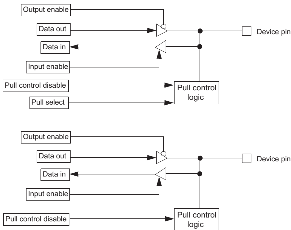
Figure 29-60. GPIO Functionality
