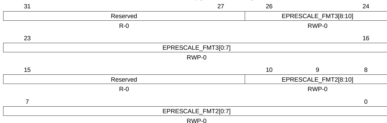
Figure 28-75. SPI Extended Prescale Register 2 (EXTENDED_PRESCALE2 for SPIFMT2 and SPIFMT3) [offset = 13Ch]
