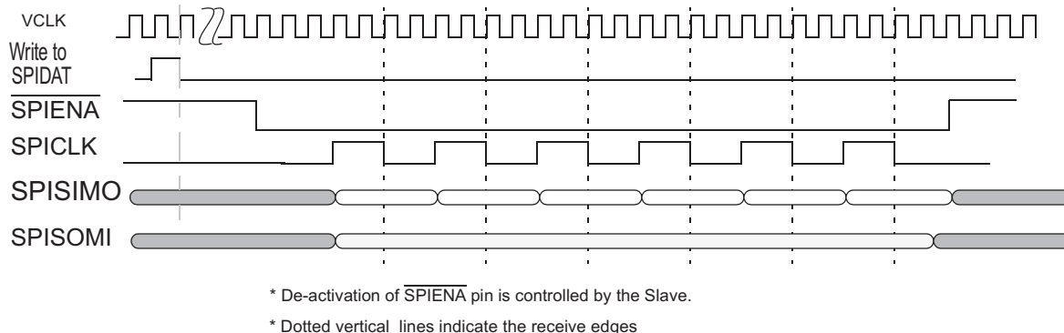
Figure 28-83. SPI/MibSPI Pins During Master Mode 4-pin with \overline{\text{SPIENA}} Configuration
