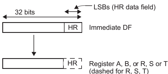
Figure 23-115. MOV32 Move Operation for IMTOREG (Case 00)
