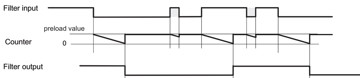
Figure 23-26. Suppression Filter Counter Operation
