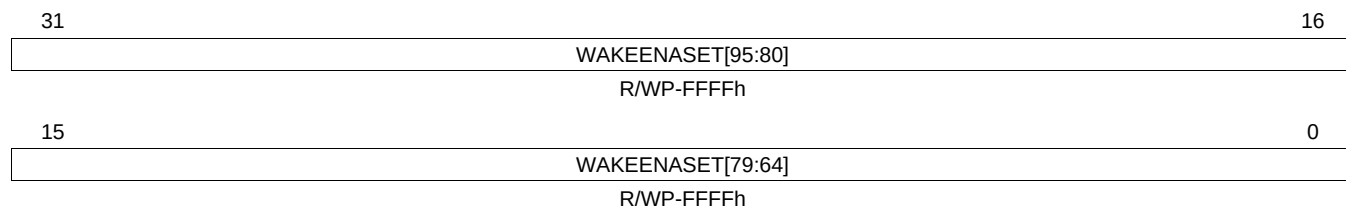
Figure 15-35. Wake-Up Enable Set Register 2 (WAKEENASET2) [Address = FFFF FE58h]
