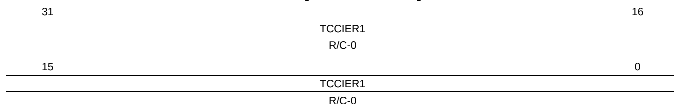
Figure 26-96. Transfer to Communication Controller Interrupt Enable Reset 1 (TCCIER1) [offset_TU = 124h]
