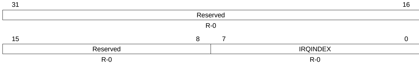
Figure 15-15. IRQ Index Offset Vector Register (IRQINDEX) [Address = FFFF FE00h]
