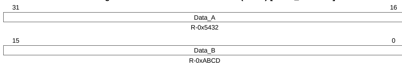
Figure 26-30. Global Static Number 0 (GSN0) [offset_TU = 00h]
