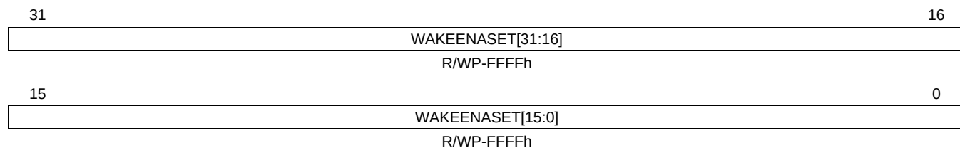
Figure 15-33. Wake-Up Enable Set Register 0 (WAKEENASET0) [Address = FFFF FE50h]
