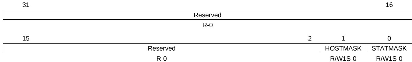
Figure 32-57. MAC Interrupt Mask Set Register (MACINTMASKSET)
