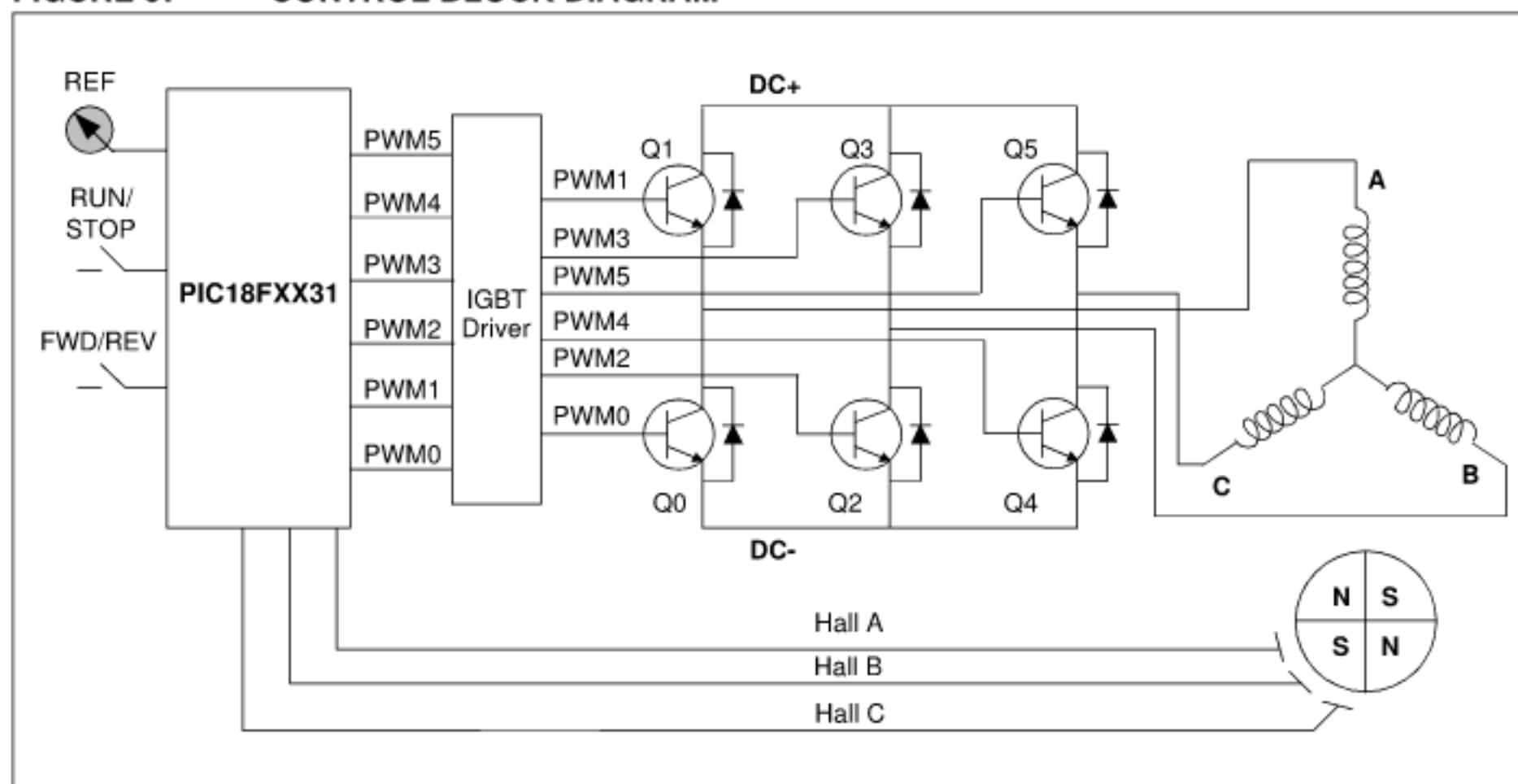
FIGURE 9: CONTROL BLOCK DIAGRAM
