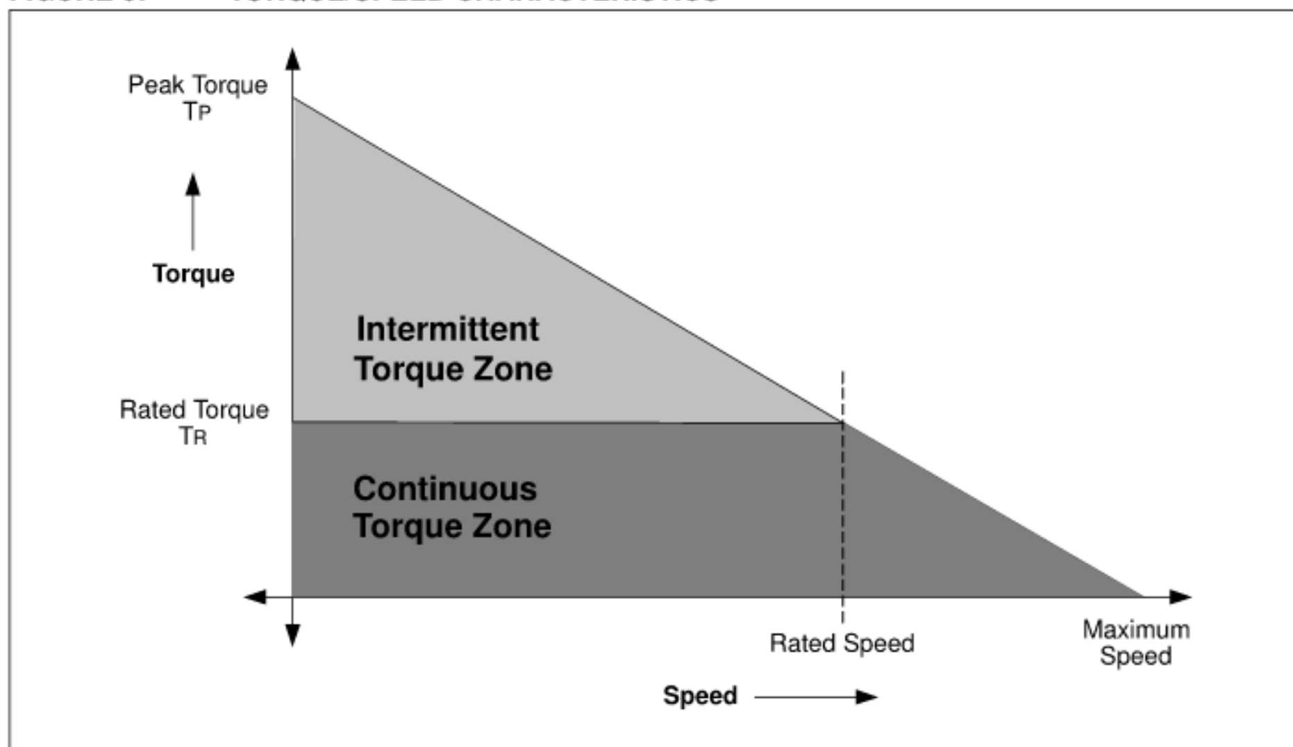
FIGURE 6: TORQUE/SPEED CHARACTERISTICS
