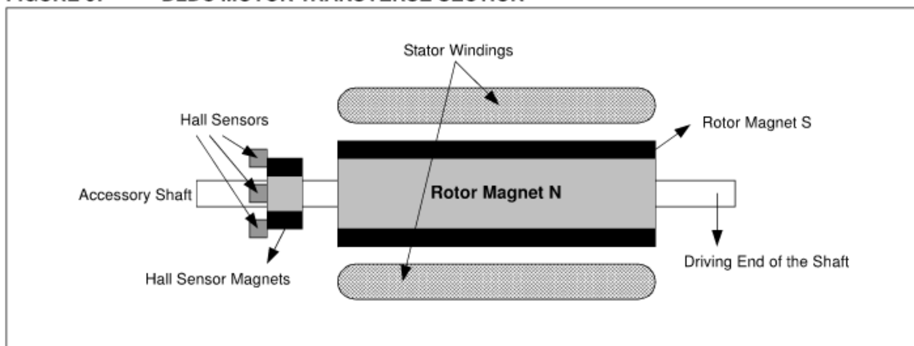
FIGURE 5: BLDC MOTOR TRANSVERSE SECTION
