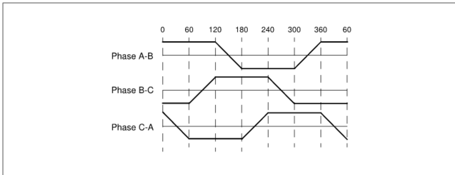
FIGURE 1: TRAPEZOIDAL BACK EMF
