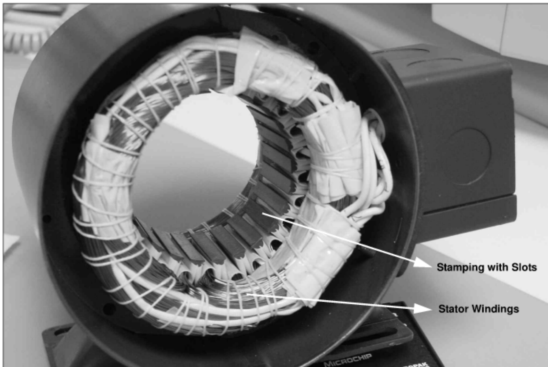
FIGURE 3: STATOR OF A BLDC MOTOR
