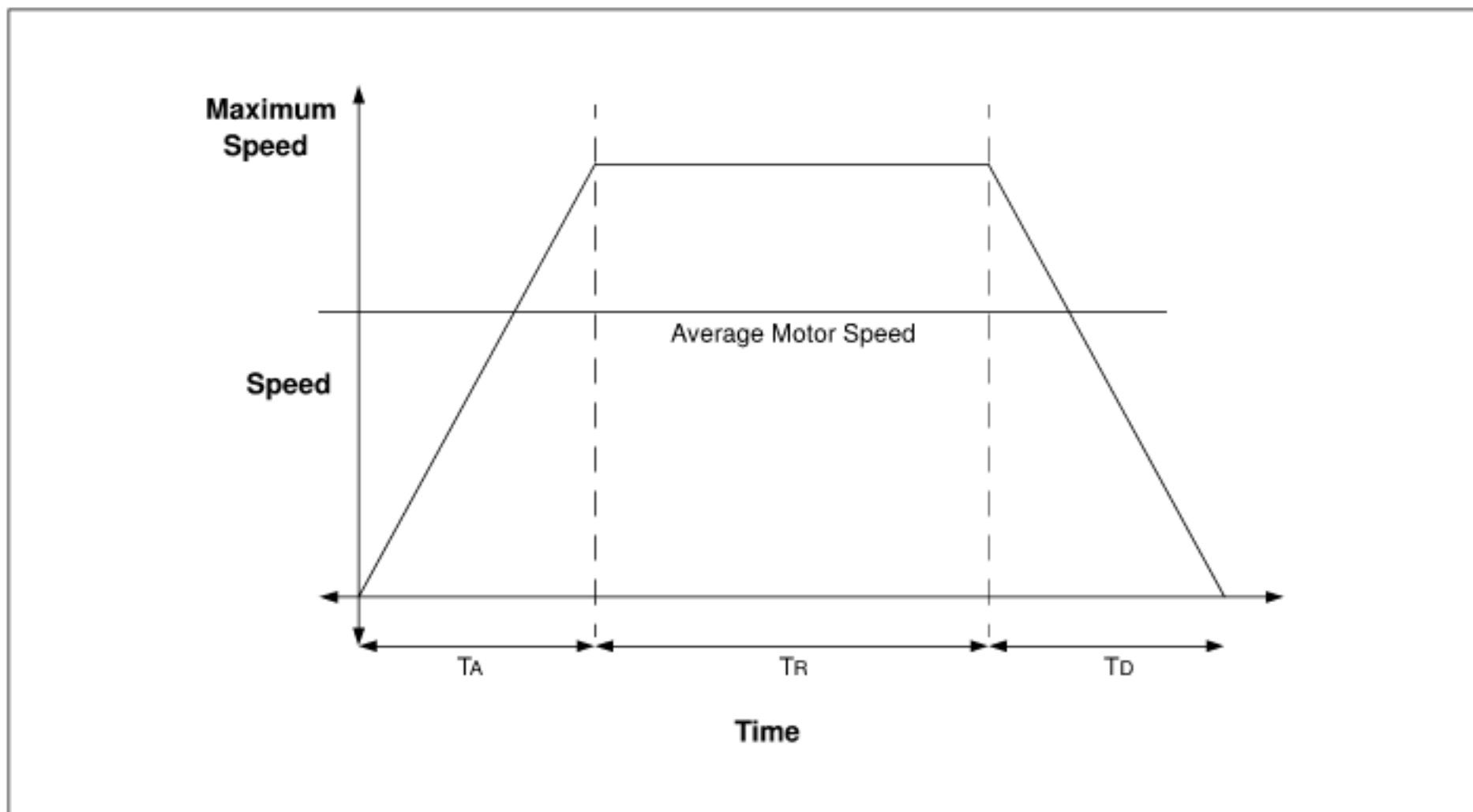
FIGURE 11: TRAPEZOIDAL SPEED CURVE
