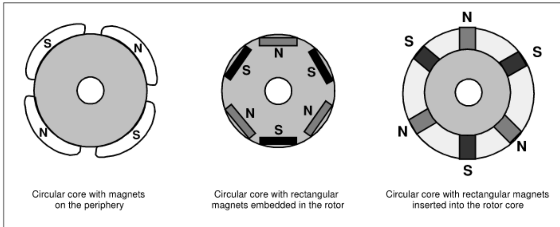
FIGURE 4: ROTOR MAGNET CROSS SECTIONS
