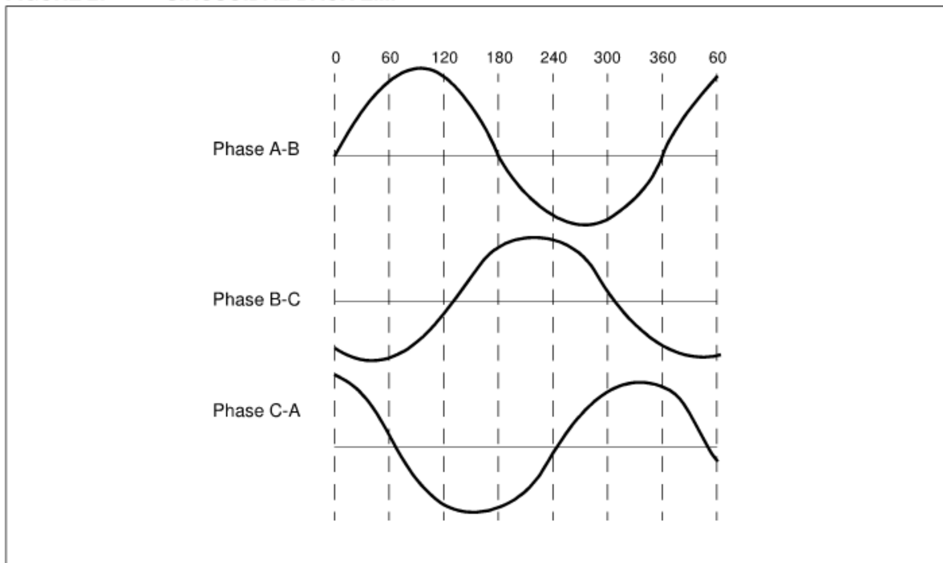
FIGURE 2: SINUSOIDAL BACK EMF
