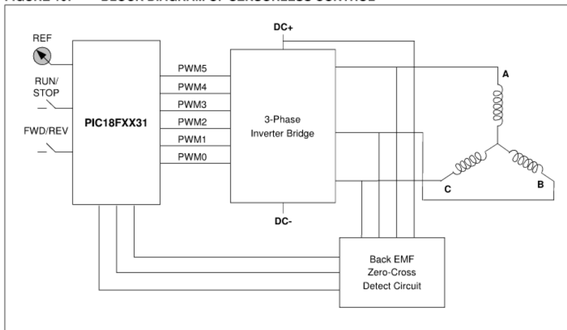
FIGURE 10: BLOCK DIAGRAM OF SENSORLESS CONTROL
