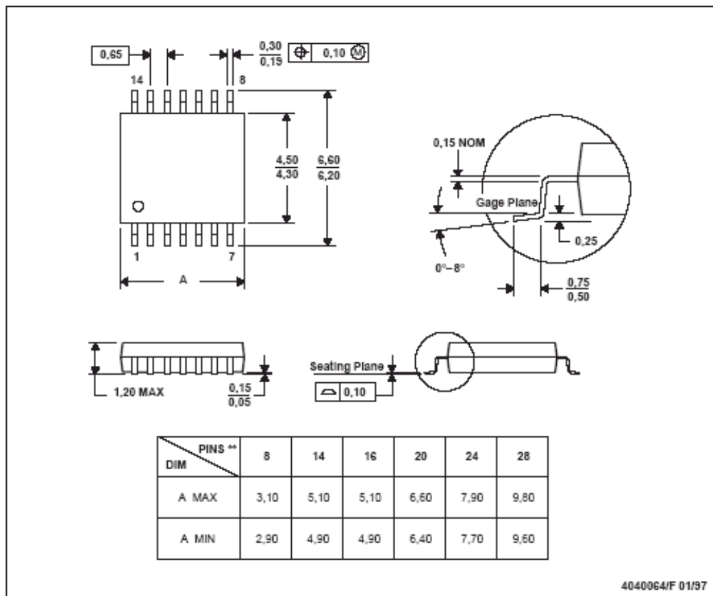
PW (R-PDSO-G**) 14 PINS SHOWN
