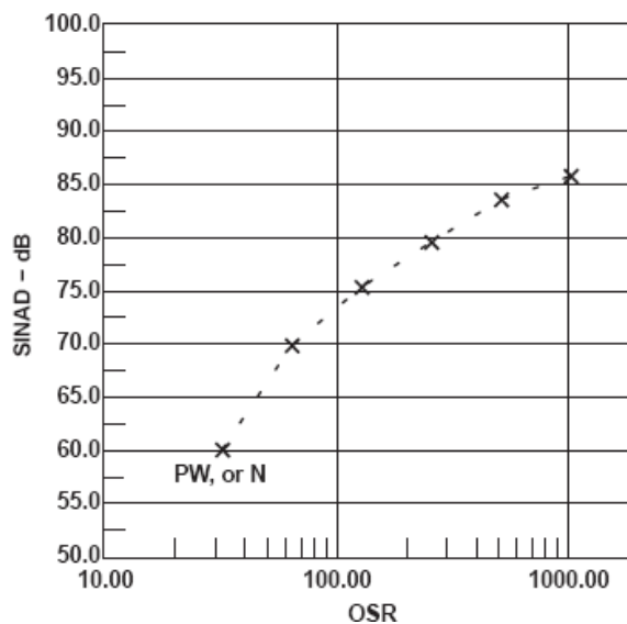
图22 SINAD VS OSR, f SD16 = 1MHz, SD16REFON = 1, SD16GAINx = 1
