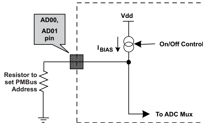
Figure 4-6. PMBus Address Detection Method
