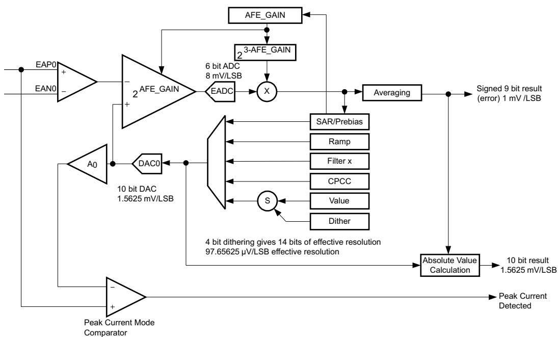
Figure 4-2. Front End Module
